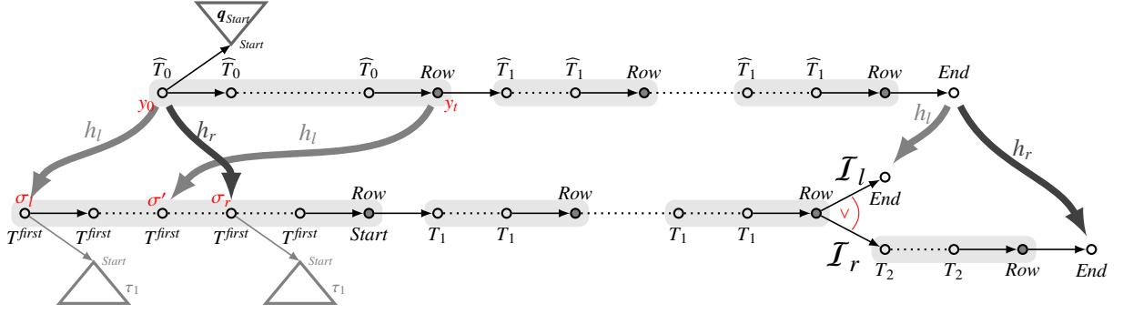
Figure 3: A query that contains both Start and End atoms must have variables with empty concept labels.
