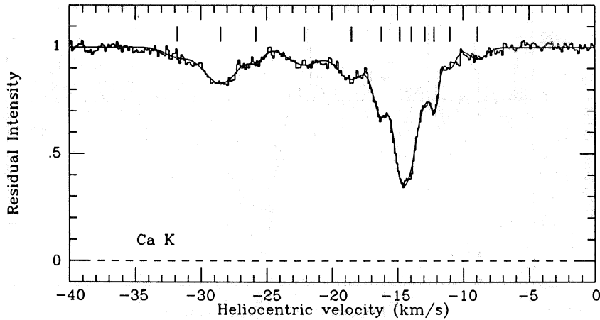
Figure 6. The interstellar Ca K line observed towards \zeta Oph. The line-profile parameters for the model fit are given in Table 2, and the velocities of the 12 identified velocity components are indicated by vertical tick marks.
