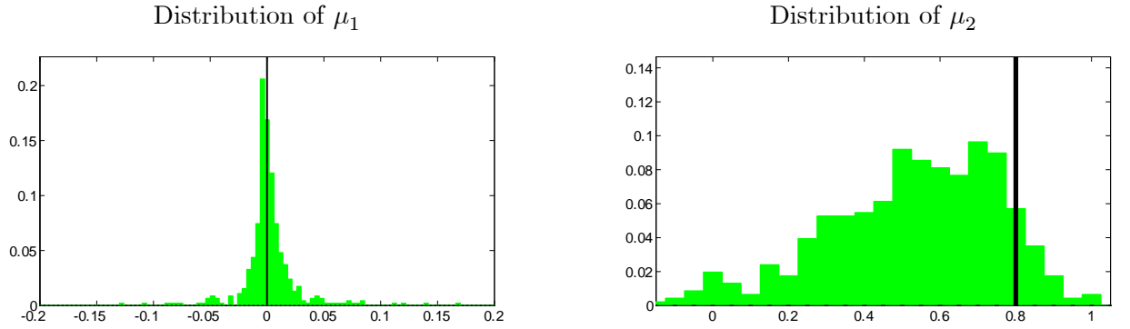
FIGURE 6. Empirical bias in the estimates of \mu_1 and \mu_2 . The light area corresponds to the histogram of the estimated NKPC parameters at the sectoral level (under \varphi > 0.5 and with the income share of intermediate goods as a proxy for the forcing variable). The black line corresponds to the estimated coefficients in the "aggregate" regression.
