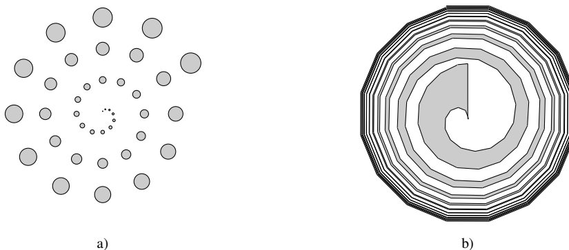
Figure 5: Non-tame regular closed subsets of \mathbb{R}^2 .
