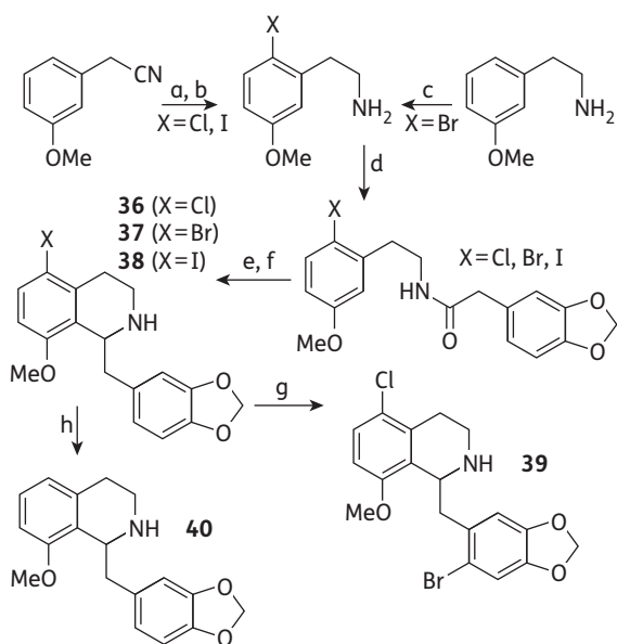
Figure 1. Bischler–Napieralski-mediated synthesis to ortho -cyclized THIs 36–40 . (a) NCS or NIS, \text{CH}_2\text{Cl}_2 ; 85% and 81% yield, respectively; (b) For X=Cl and I, \text{B}_2\text{H}_6\cdot\text{SMe}_2 , 42% and 55%, respectively. (c) \text{Br}_2 , \text{CH}_3\text{CO}_2\text{H} , 67%. (d) 3,4-(Methylenedioxy)phenylethanoic acid, N,N -dicyclohexylcarbodiimide (DCC), 4-dimethylaminopyridine (DMAP), \text{CH}_2\text{Cl}_2 ; X=Cl and X=Br, 99%, X=I, 74%. (e) \text{POCl}_3 , toluene, reflux. (f) \text{NaBH}_3\text{CN} , MeOH; 36 19%, 37 19%, 38 2% over two steps. (g) 36 , NBS, \text{CH}_2\text{Cl}_2 , 35%. (h) 37 , \text{LiAlH}_4 , -78^\circ\text{C} , 89%.
