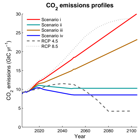
Figure 3. Total CO 2 emissions associated with four different electricity sector-only policy scenarios. Total CO 2 emissions associated with two RCPs are shown for reference. (Note that the RCP scenarios cover all sectors and land use.)
