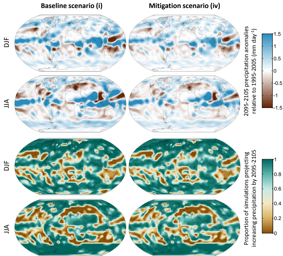
Figure 6. 2095–2105 precipitation anomalies (ensemble means) relative to 1995–2005 under the baseline scenario i, and the mitigation scenario iv (top panels) and proportion of ensemble members simulating increased precipitation (bottom panels).
