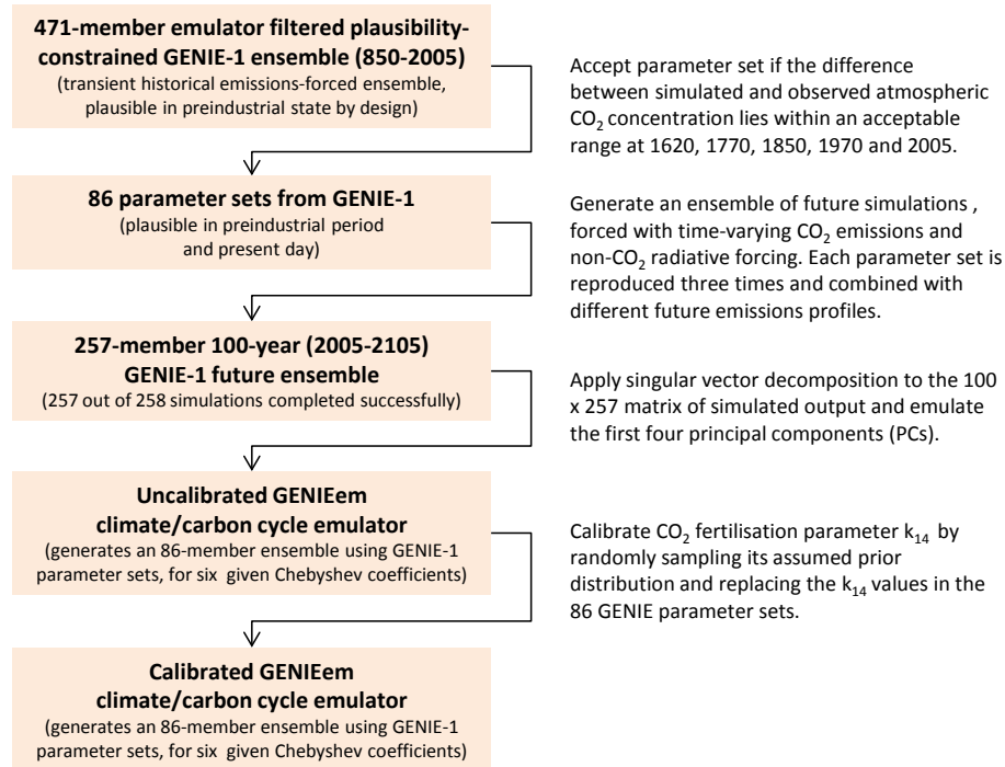
Figure 1. Schematic describing the construction of GENIEem.
