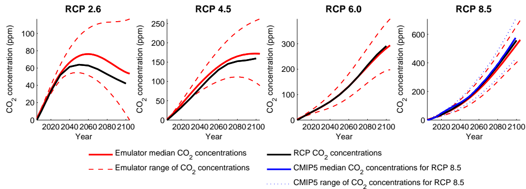
Figure 2. Carbon cycle emulator output compared with RCP data, for the four RCPs 2.6, 4.5, 6.0 and 8.5. Anomalies are relative to 2005. For RCP8.5, CMIP5 data are presented as a reference.
