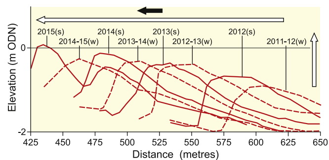
Fig. 10. Vertical and lateral intertidal bar migration at Holkham Bay between six-monthly winter (w) and summer (s) surveys, 2012–2015 for a representative cross-shore profile (EA reference number N024). The time period affected by the 5th December 2013 storm surge is shown by the uppermost horizontal arrow.
