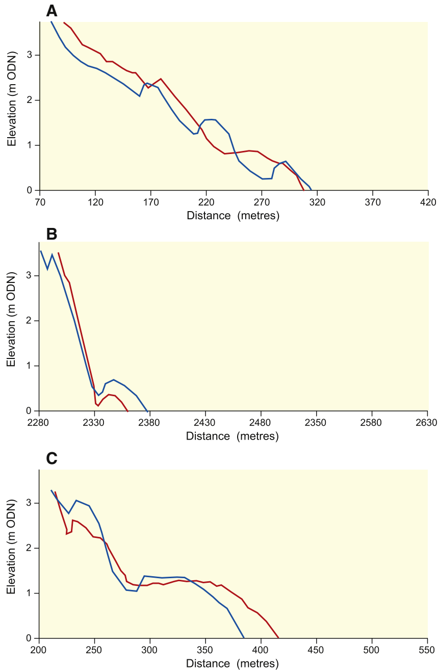
Fig. 7. Cross-shore profiles between 0 m ODN and MHWS for 2008 and 2013 for A) Brancaster Bay (at EA cross-shore profile N008); B) Scolt Head Island (N015); and C) Holkham Bay (N024).
