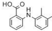
mefenamic acid
