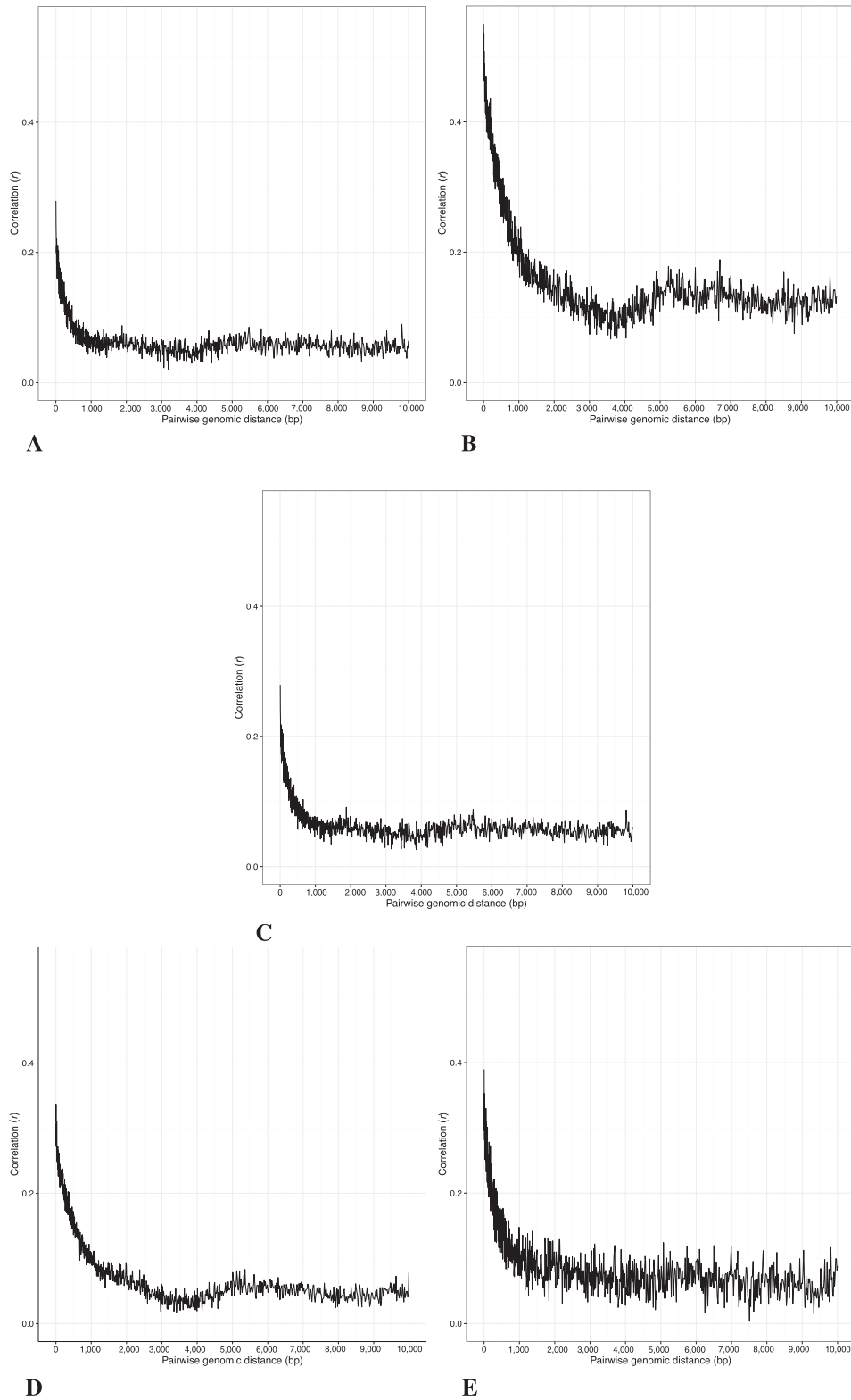
FIGURE 1 Correlation versus genomic distance for pairs of probes in chromosome 1 Notes: (A) Gambian, (B) CRC, (C) Caucasian, (D) Afr-Am-GTP, (E) Cau-Am.
