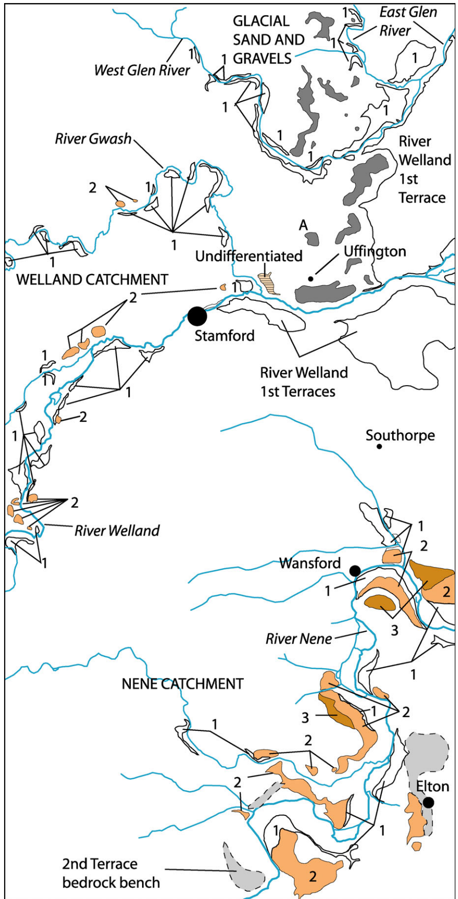
FIGURE 3 Distribution of glacial sands and gravels north of the River Welland as well as Nene and Welland fluvial terraces relevant to the sites studied (Redrawn from BGS, 1976, 1978, 1984)
