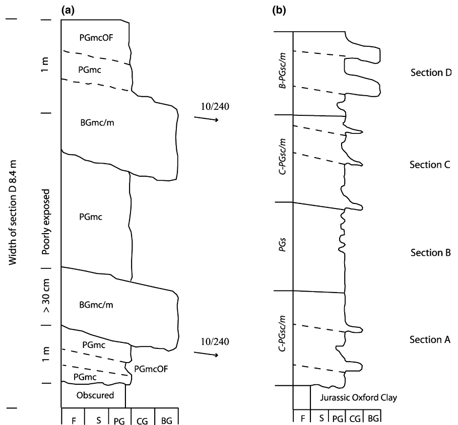
FIGURE 8 (a) Idealized lithological log for section D at Uffington. Note that this is not a vertical succession but represents lateral aggradation over about 8.4 m. Only the upper 1 m of parts of section D was clearly exposed. Only two beds of facies BGmc/m appeared to be present but their thickness could not be ascertained. (b) Simplified stratigraphical log based on observations from sections A–D
