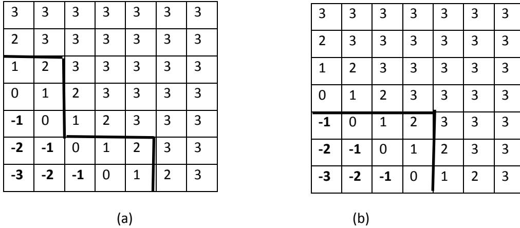
Figure 2. Values c_{ij} - (p-1)/2 for the blocks of the consensus matrix for the Likert scale consensus problem when p = 7 . The bold line represents the boundary separating entries summed in criterion (12), i.e. those above and to the right of it, from the rest. Fig.2 (a) shows the case in which the seven parts are merged into three aggregated parts: (i) the first two parts, (ii) the next three parts, and (iii) the last two parts. Fig. 2(b) shows the case in which the seven parts are merged into two aggregated parts: (i) the first four parts, and (ii) the last three parts.
