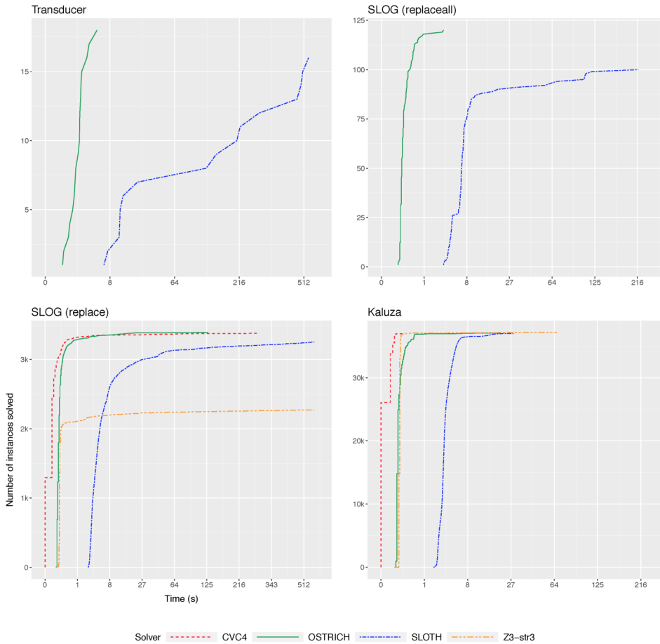
Fig. 4. Comparison of solvers on several sets of benchmarks.
