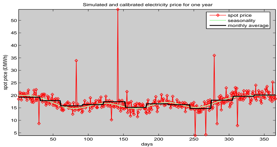
Figure 8: Simulated price path.
