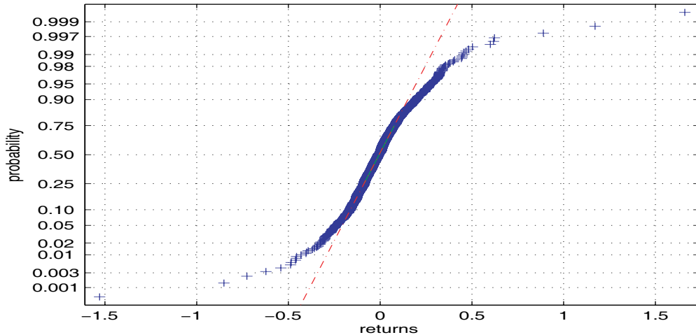
Figure 3: Normal probability test for returns of electricity prices from 2/04/01 to 3/03/04.
