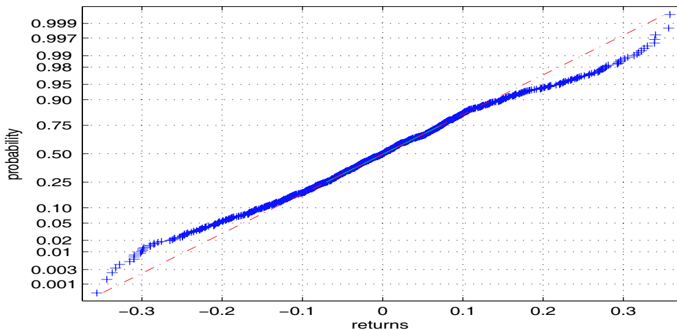
Figure 6: Normal probability test for filtered returns of electricity prices.
