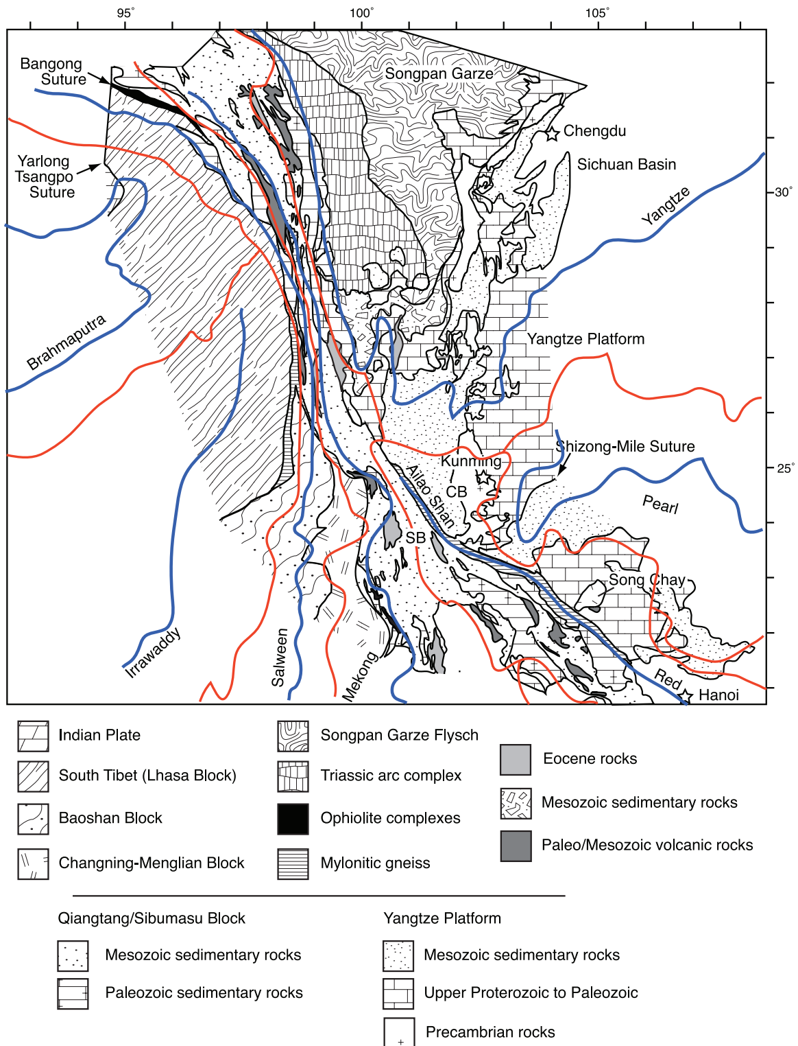
Figure 3. Regional geological map of the eastern Tibetan Plateau, SW China, and northern Indochina showing the river courses overlain in blue and the extent of the drainage basins in red. Map redrawn from original provided by B. C. Burchfiel (unpublished data, 2006). CB, Chuxiong Basin; SB, Simao Basin.
