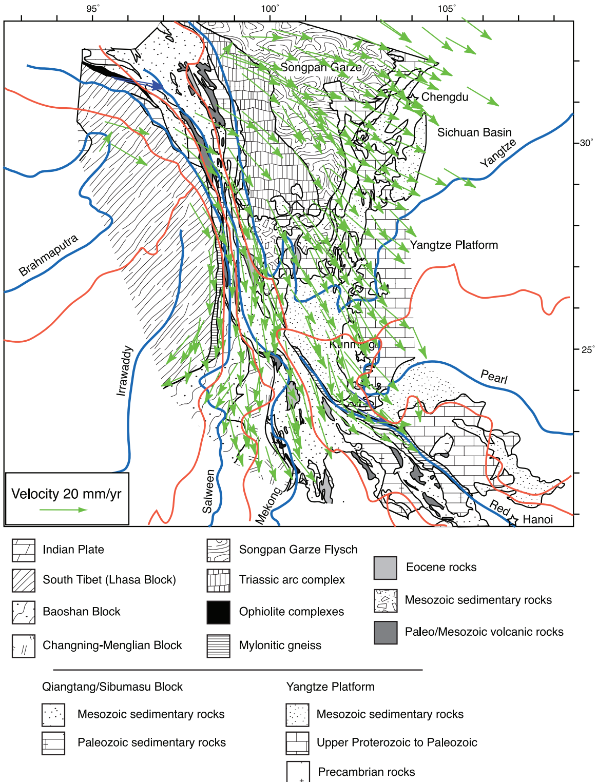
Figure 13. Map showing the geology of eastern Tibetan Plateau, SW China, and northern Indochina overlain by arrows showing the present-day rates of horizontal crustal motion relative to a stable Eurasia continent, measured by GPS [Chen et al. , 2000] and modeled by Meade [2006]. Rivers are shown as blue lines, with the edge of their drainage basins shown in red.
