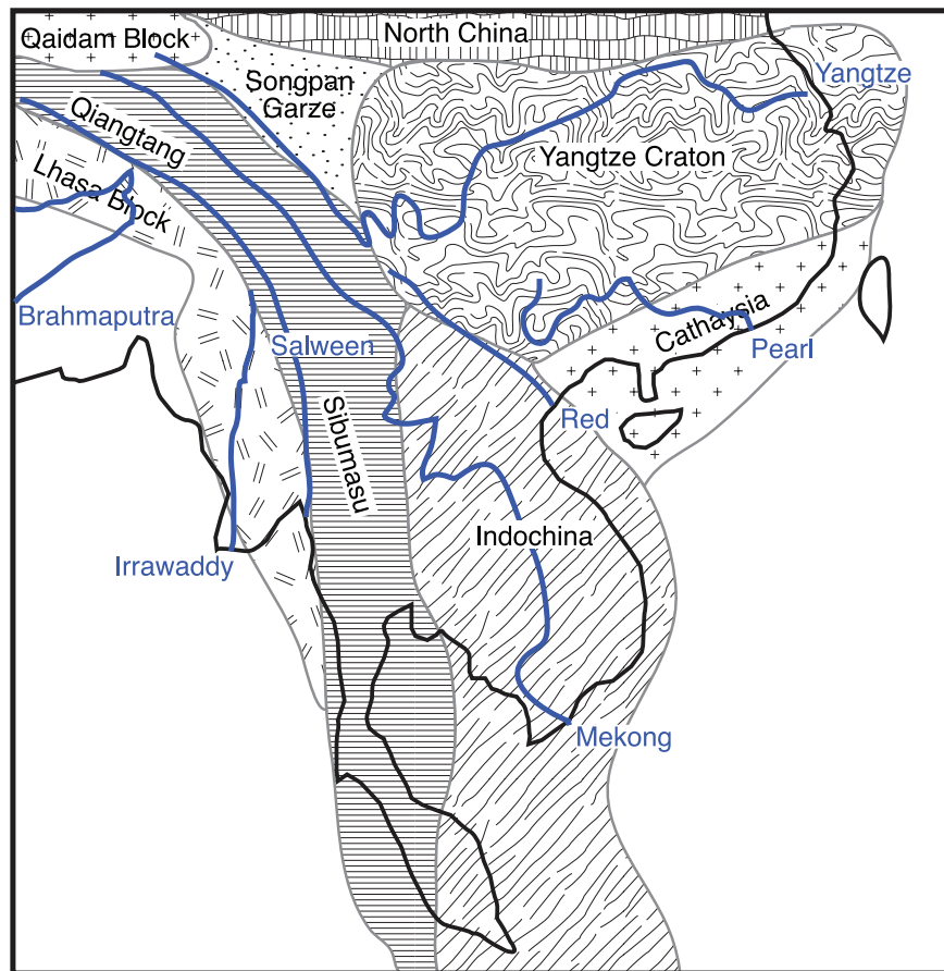
Figure 2. Simplified tectonic terrane map of East and Southeast Asia showing the major blocks discussed in this paper [after Metcalf , 1996] and the courses of the rivers colored in blue.
