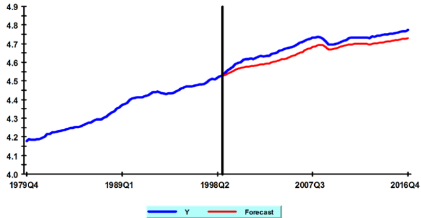
Plot of Actual and Single Equation Dynamic Forecast(s) of Y
