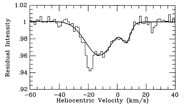
Figure 3. The interstellar Na I D 2 line towards \alpha Pav observed from ESO ( R = 80\,000 ). Note the narrow interstellar D 2 line superimposed on the photospheric C II \lambda 5889.79 line. The smooth curve is a two-component Gaussian fit to the stellar lines, and defines the local continuum for the interstellar line.
