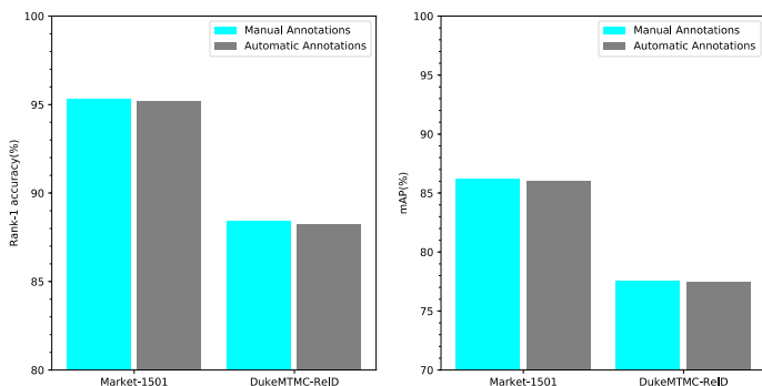
Fig. 10. Performance comparison of CDPM with automatic annotations and manual annotations.
