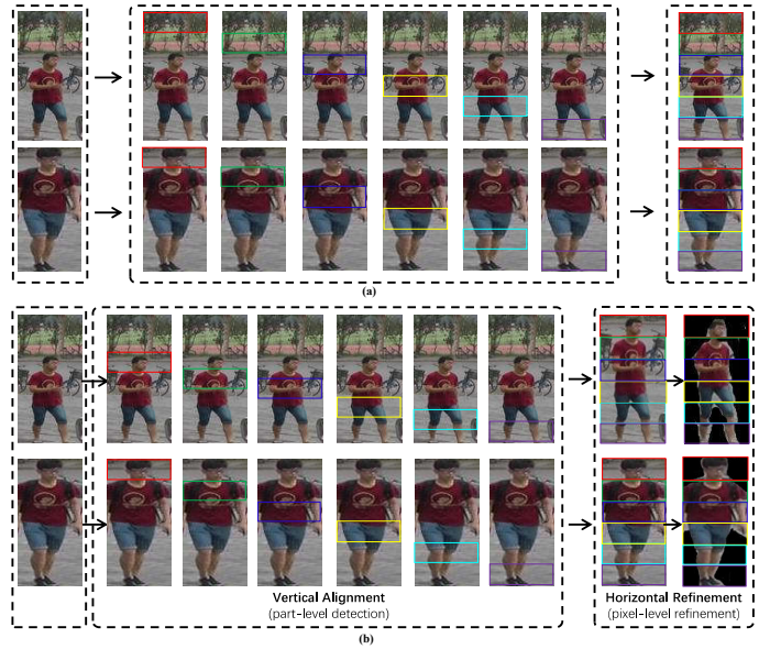
Fig. 1. (a) The pipeline of the baseline model based on uniform division [7]. The severe part misalignment problem dramatically degrades the quality of the part-level representations. (b) The inference pipeline of CDPM. It decouples the part alignment problem into two easier steps, i.e., a vertical alignment step and a horizontal refinement step. In this way, body parts are semantically aligned across images. Best viewed in color.
