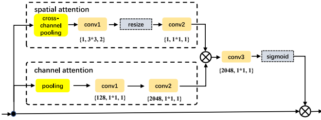
Fig. 6. Architecture of the Spatial-Channel Attention (SCA) model [6]. We utilize SCA to realize the horizontal refinement operation. The three items in each bracket are filter number, kernel size, and stride. In the interests of brevity, the BN and ReLU layers after each convolutional layer are not shown here. The value of all hyper-parameters of SCA remains the same as in [6].
