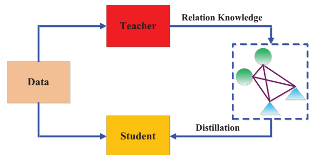
Fig. 13 A generic framework for graph-based distillation.
