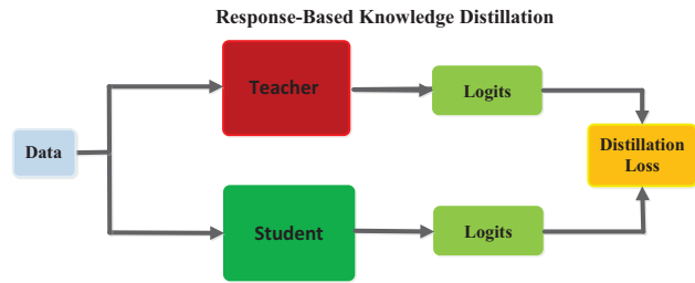
Fig. 4 The generic response-based knowledge distillation.
