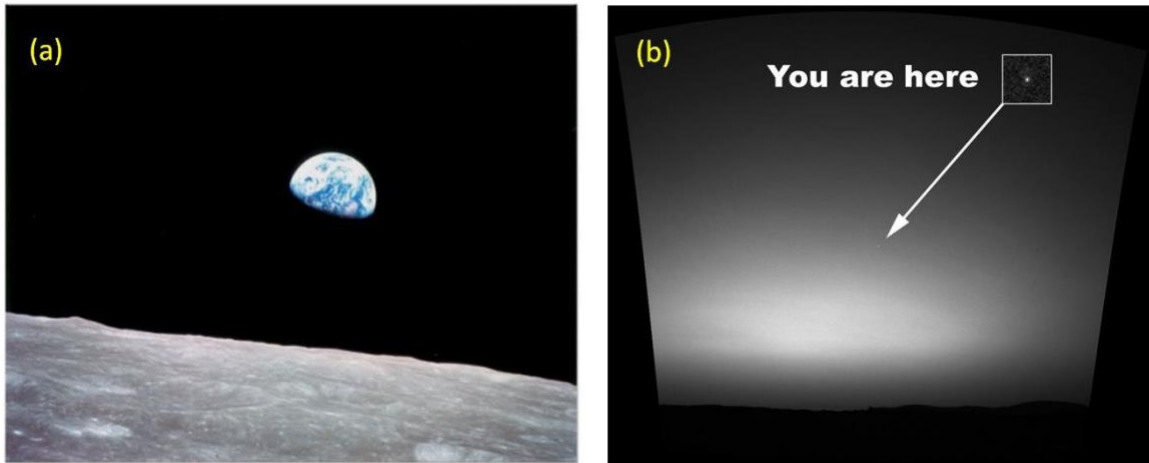
Figure 1. (a) Earthrise over the lunar surface, photographed by the crew of Apollo 8 in December 1968. (b) The Earth photographed from the surface of Mars by the Mars Exploration Rover ‘Spirit’ in March 2004. Such images powerfully reinforce a ‘cosmic perspective’ that can help build a sense of human community. Images courtesy of NASA.
