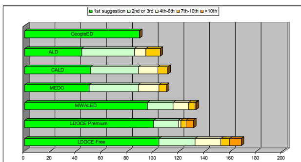
Figure 2: Performance of the seven dictionaries for all data (N=202). Colour bars indicate the number of target words ranked in the respective positions in the suggestions list.
