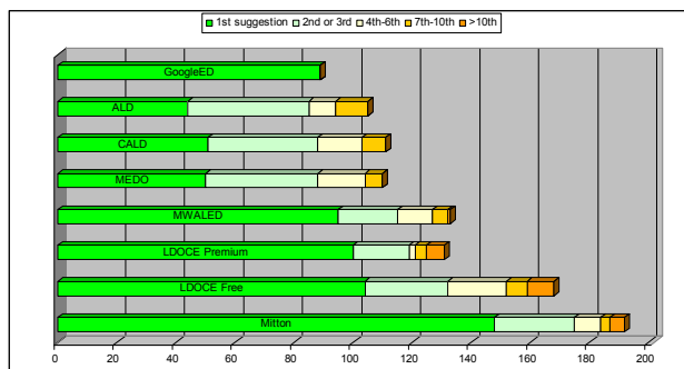
Figure 5: Performance of the seven dictionaries compared with Mitton’s experimental spellchecker, for all data (N=202)
