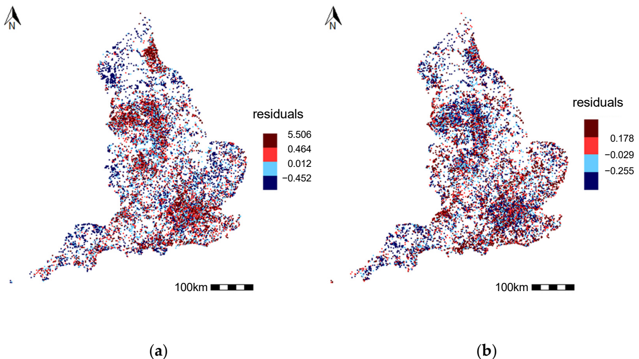
Figure 4. Residuals of the OLS regression plotted for (a) the l_{sps} model and (b) the l_{val} model.
