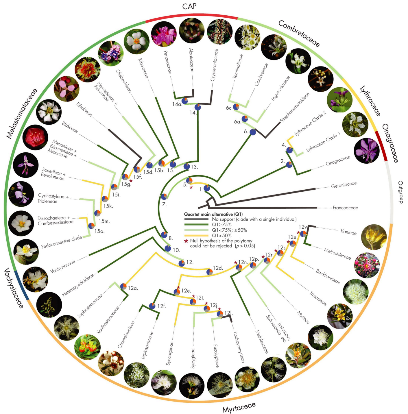
FIGURE 2. Coalescent astral tree summary showing relationships in key Myrtales families and subclades, using exons, inferred in ASTRAL. Pies charts on branches display quartet score (QS) values as described for Fig. 1A. Branches and clade color code follow the quartet main topology (Q1) support value, with dark green \geq 0.75 ; light green \geq 0.50 , < 0.75 ; and yellow < 0.50 . Red asterisks next to pie charts indicate the null hypothesis of a polytomy (equal support for species tree, first alternative, and second alternative topology) could not be rejected with the polytomy test ( p > 0.05 ). Numbers on branches relate to clades reported in Appendix S4. Photo credits: Counter clockwise from Onagraceae: OFS, WMC, ST, DH, OM ( \times 3 ), JD, PM, OM, DP ( \times 3 ), FM, DP, FM, DP, FM ( \times 3 ), GS, OM, OFS, YP, PW, FF, CSIRO, EL, OFS, CSIRO, RBGK, TV, FF ( \times 2 ), DD, EL, WT. Commonwealth Scientific and Industrial Research Organisation (CSIRO); D. Dixon (DD); J. Dransfield (JD); F. Forest (FF); O. Fragman-Sapir (OFS); D. Harris (DH); P. Maas (PM); O. Maurin (OM); W. McClelland (WMC); E. Lucas (EL); F. Michelangeli (FM); D. Penneys (DP); Y. Pillon (YP); Royal Botanic Gardens, Kew (RBGK); G. Shimizu (GS); W. Takeuchi (WT); S. Turner (ST); T. Vasconcelos (TV) and P. Wilson (PW).
