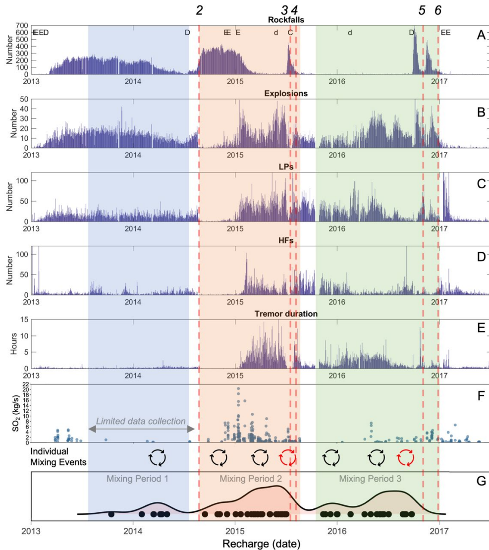
Fig. 8. Seismic (A–E) and gas (F) monitoring data compared to the timeline of mixing events (density curve of all data, G). Coloured transparent boxes as in Fig. 6. Circular arrows above the density plot refer to inferred individual mixing events based on peaks in the density distributions and clusters of data, representing in-dividual mixing events within a broader recharge period, with black circles represent priming injections and red circles representing triggering injections. Red dashed lines represent the start date of the eruption (cf. the red fields in Figs. 6 and 7) with the Eruptive Phase marked as the italicised number on the top of the line. (For interpretation of the references to colour in this figure legend, the reader is referred to the web version of this article.
