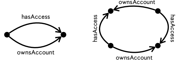
Figure 2: Two graphs indistinguishable by ShEx
