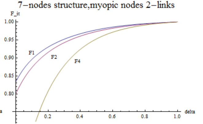
Figure 2.25: \bar{F} centrality for the 7 nodes structure with myopic nodes (2 links sight).
