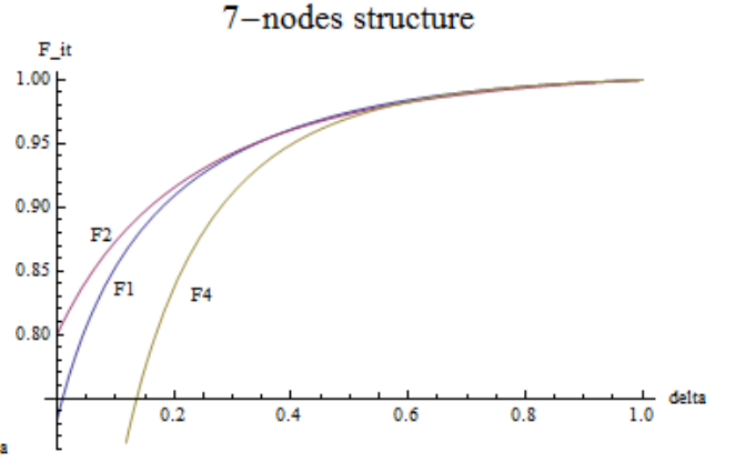
Figure 2.23: \bar{F} centrality for the 7 nodes structure.
