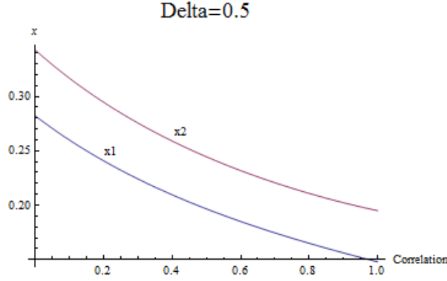
Figure 2.4: 3 nodes Star with positive asset-correlation and \delta = 0.5 .
