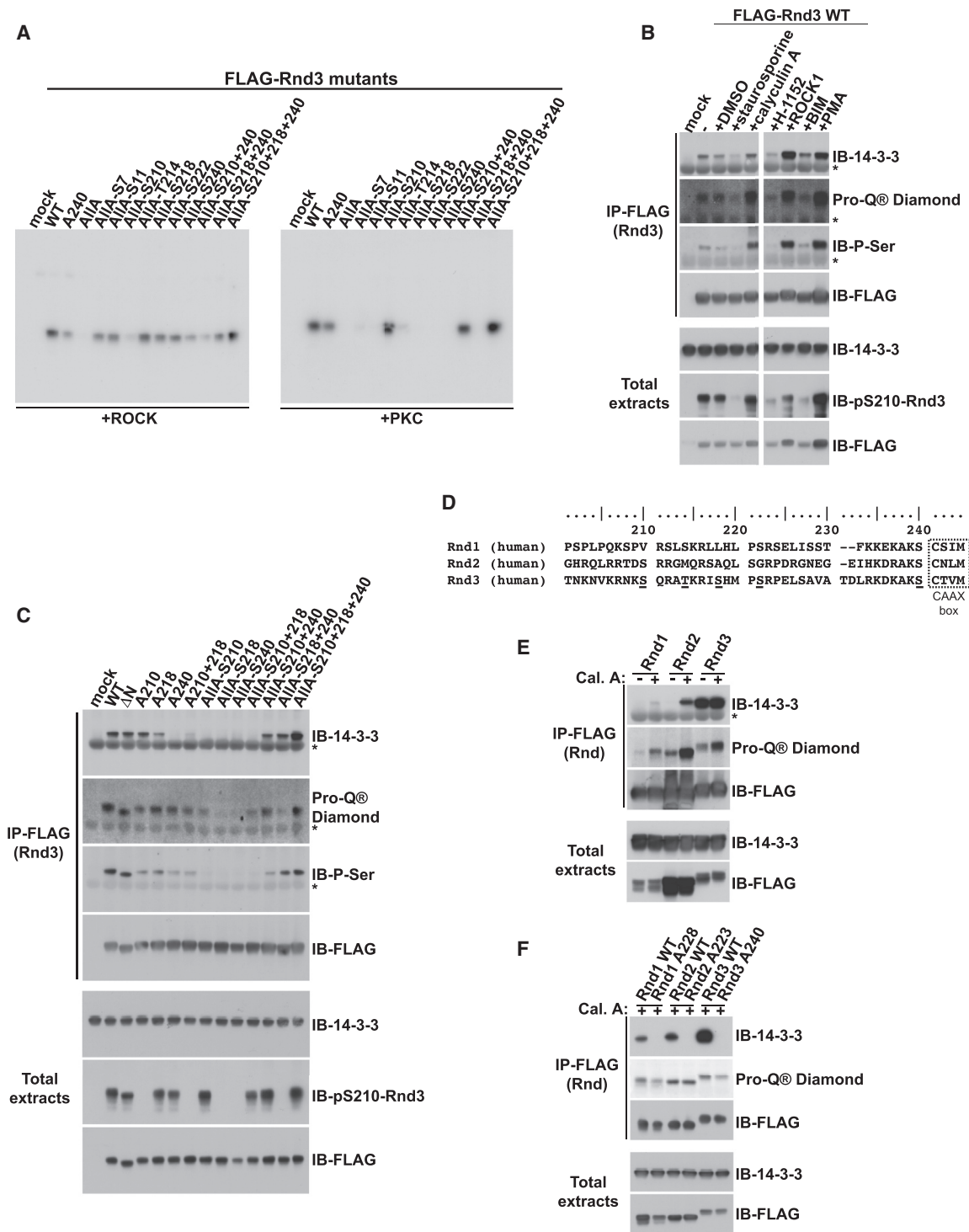
Figure 2. Rnd3 C-Terminal Phosphorylation by ROCK and PKC Is Required for 14-3-3 Interaction (A–C) The indicated constructs were transfected into COS7 cells. Cell lysates were immunoprecipitated with FLAG antibody. (A) Immunoprecipitates were subjected to an in vitro kinase assay with either ROCK1 or PKC \zeta kinase domains. (B) FLAG-Rnd3 was co-overexpressed with ROCK1 1–420 where indicated. Cells were treated with chemical inhibitors (staurosporine, calyculin A, H-1152 [ROCK], BIM1 [PKC]) or the chemical activator PMA (PKC) for 2 hr (20 min for calyculin A) prior to lysis. Cell lysates were stained with Pro-Q Diamond reagent or immunoblotted with the indicated antibodies. The space in the gel image marks the position of lanes that were not germane to these results and were thus removed during figure preparation for clarity. (C) Endogenous 14-3-3 proteins were detected with anti-14-3-3 antibody. Membranes were also stained with Pro-Q Diamond reagent or immunoblotted with the indicated antibodies.
