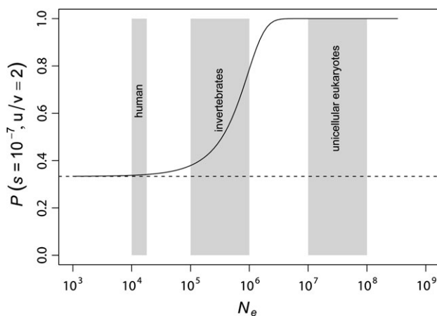
FIG. 1.—Theoretical expected equilibrium frequency ( P ) of an optimal codon versus effective population size ( N_e ). The curve represented in the figure is from rearranging equation (1). The gray rectangles show estimated effective population size intervals for some eukaryotic groups (Sherry et al. 1997; Harpending et al. 1998; Lynch and Conery 2003). Estimates of selection on codon usage are in the order of 10^{-6} to 10^{-9} (Hartl et al. 1994; Maside et al. 2004). A value of s = 10^{-7} was chosen for illustrative purposes only. The dashed line shows the equilibrium frequency of the codon under no selection when u/v = 2 .
